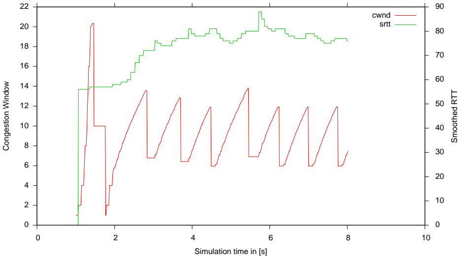
NewReno TCP Congestion Control Simulation
